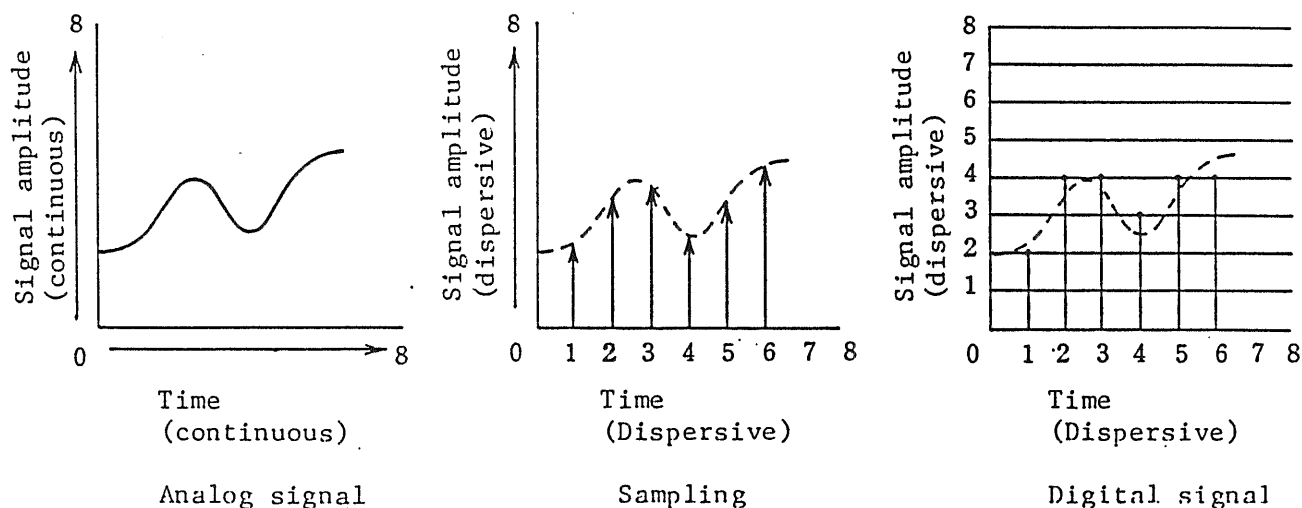
Figure 7-2. A/D Converter
